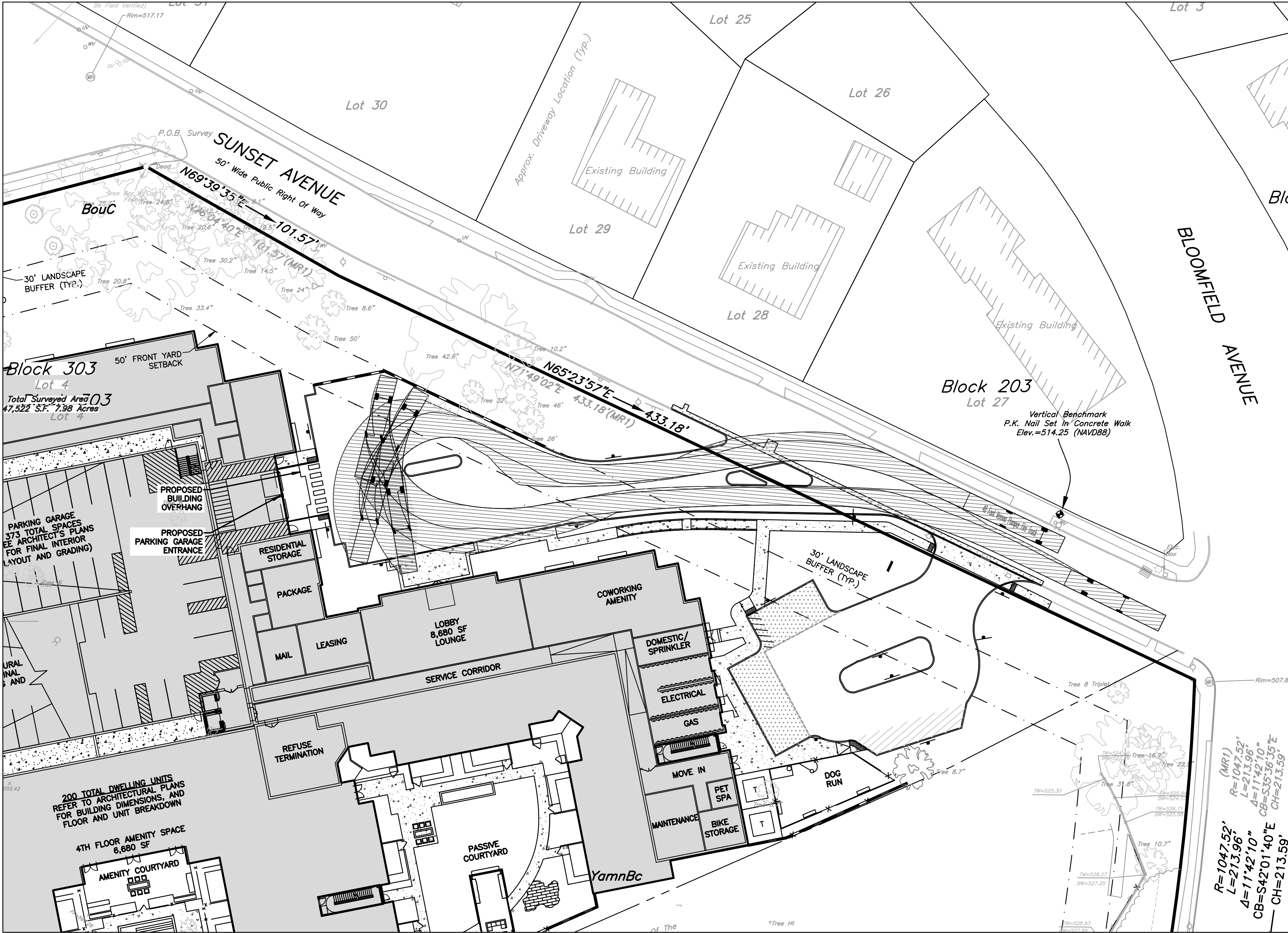
VERONA FIRE TRUCK TURNING PLAN SCALE 1" = 30'
