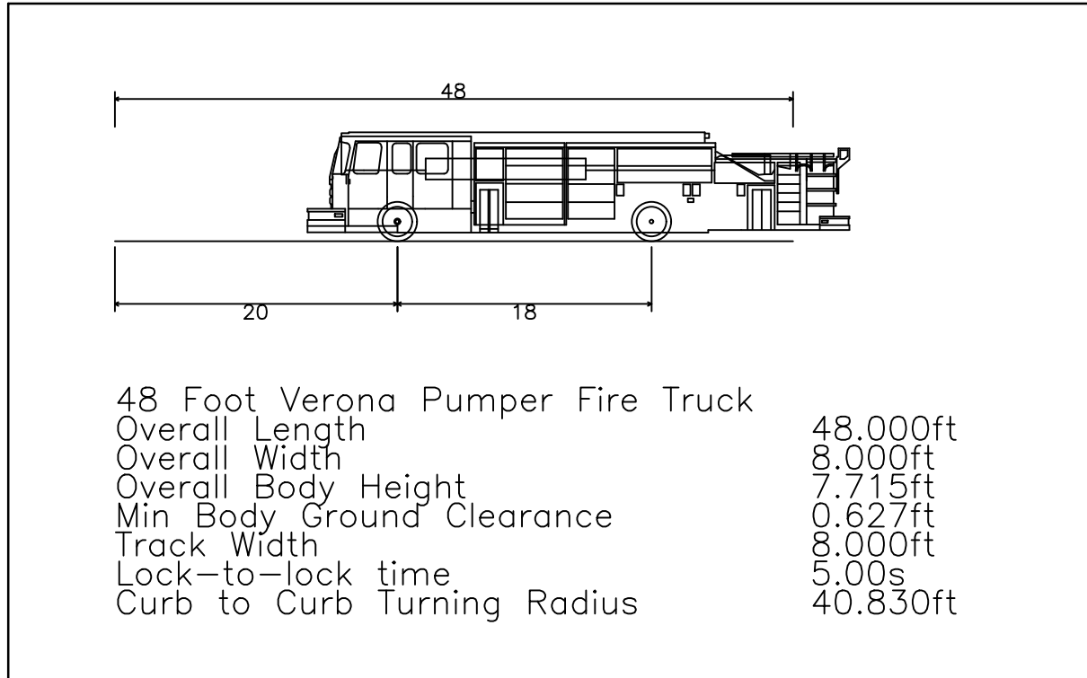
VERONA PUMPER FIRE TRUCK DETAIL NOT TO SCALE
